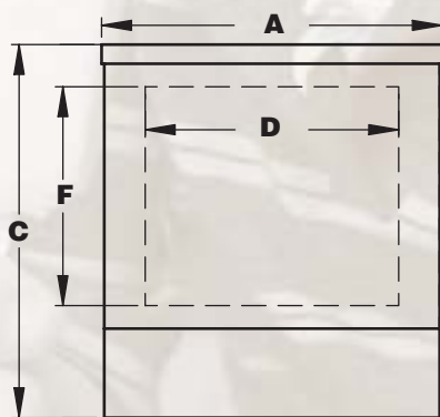
HSD/SC/P Plan View
