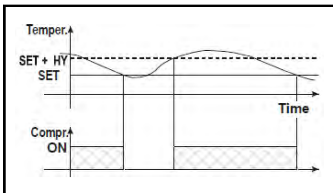
Figure 3-1 - Compressor Temperature Regulation
