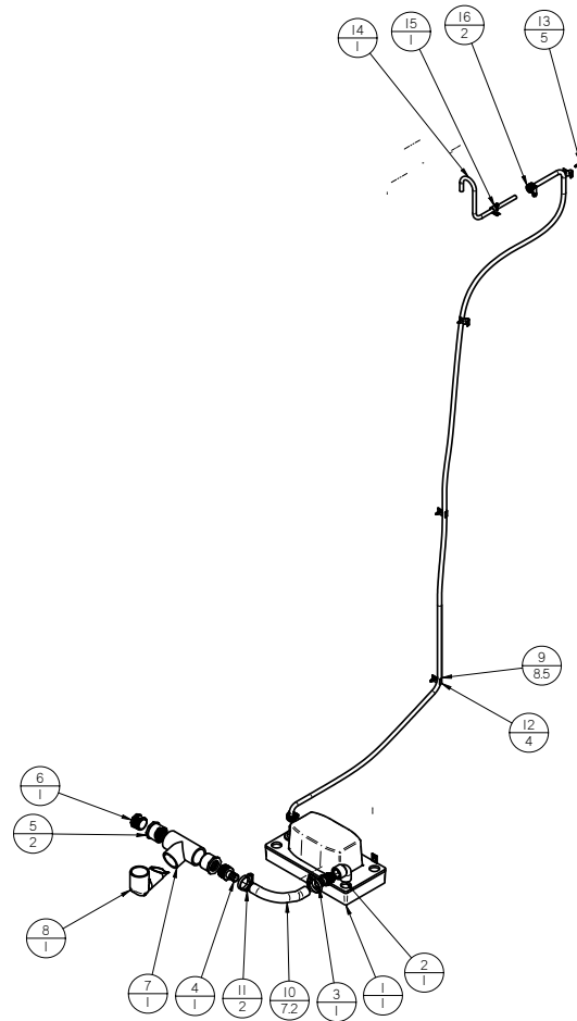
EXPLODED VIEW 1.8
