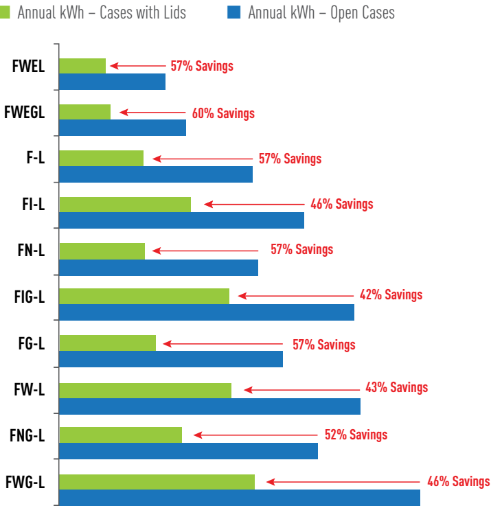
Annual kWh Comparison: Open Cases vs Cases with Lids
