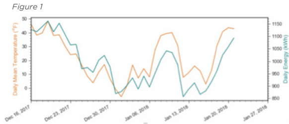
Using the 35-day window to compare Daily Mean Temperature and Daily Energy, it was found to be a highly correlated relationship and was then used as the baseline for the weather-normalized energy savings calculations.
