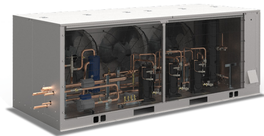
Shown: Proto-Aire EZ Multi-Compressor Distributed System
