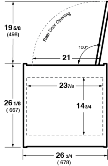
Plan View
