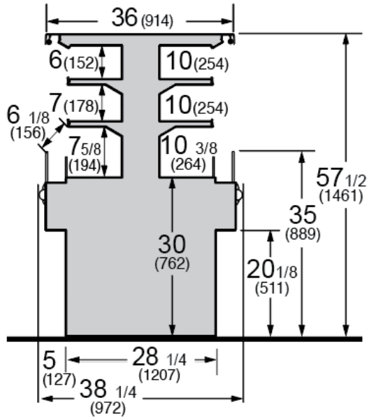
Cross section
