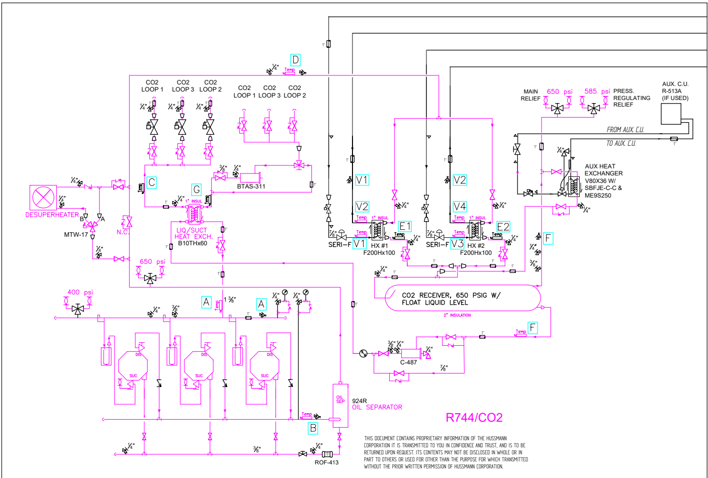
TYPICAL CO2 CASCADE PIPING (See following page for right side of diagram.)
