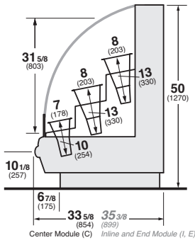
IM-05-RF-NC Refrigerated Self-Service Floral with narrow canopy
