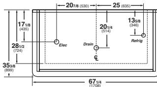
IM-04-E5-R, IM-05-E5-R End Module
