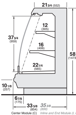
IM-04-E5-R, IM-05-E5-R End Module
