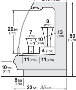
IM-05-RF Refrigerated Self-Service Floral Module
