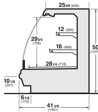
extended deck (IM-04-ED6-R)
