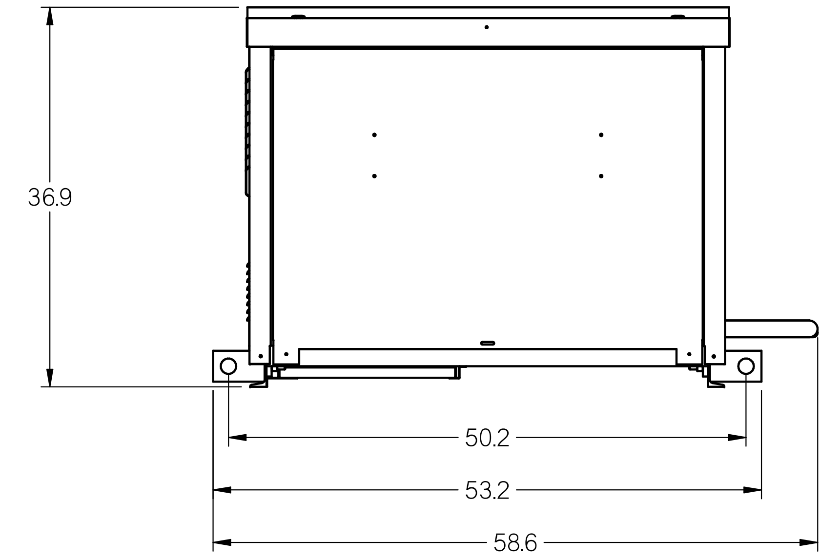
Side View
