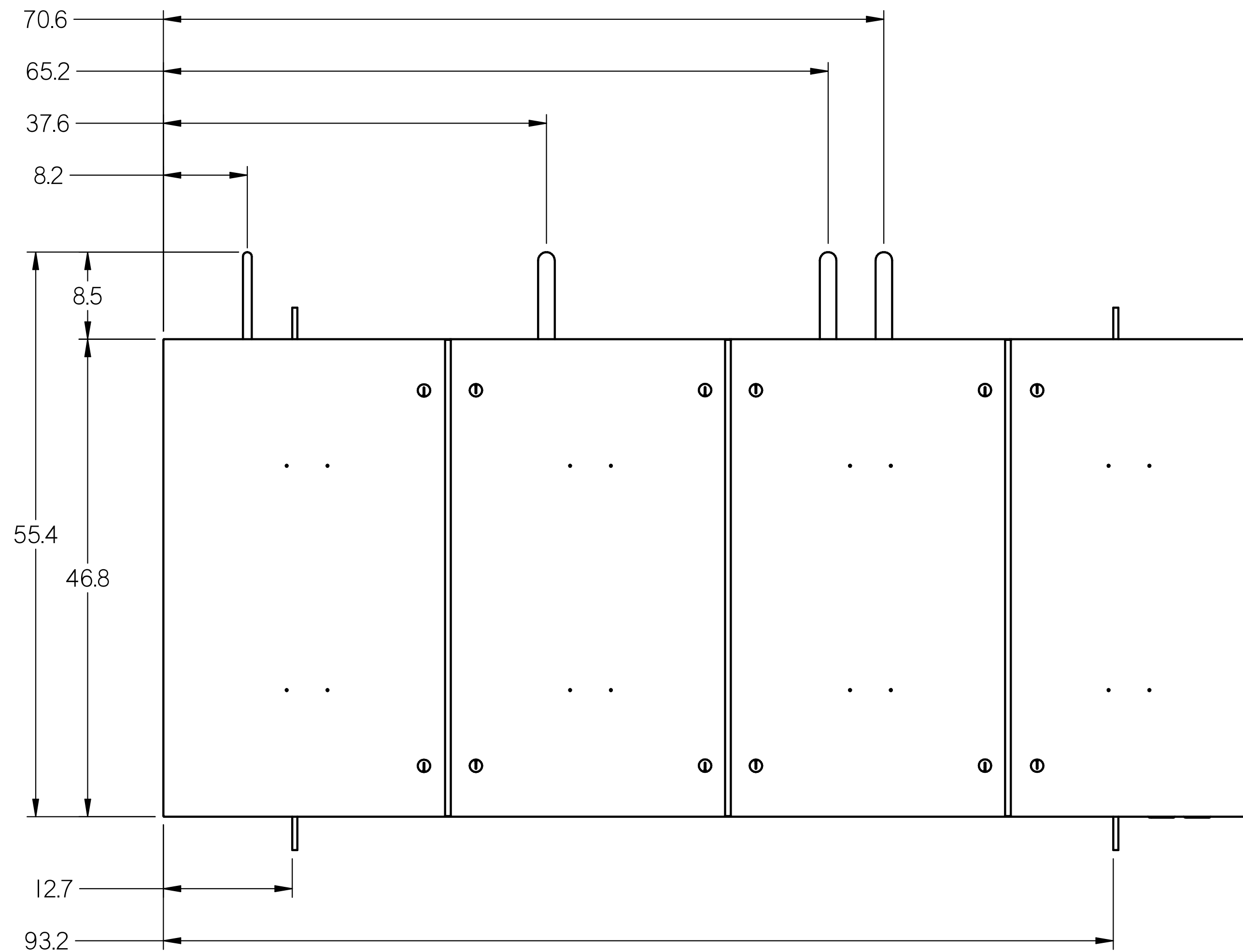
Plan View
