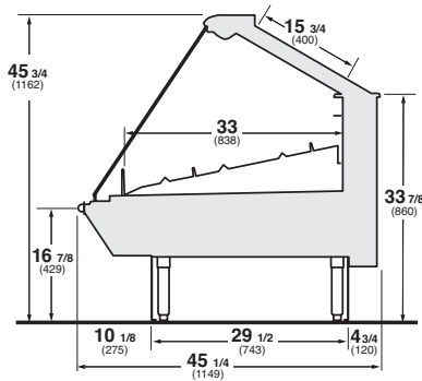
Q1-FS Straight Glass - Single-Deck Fish
