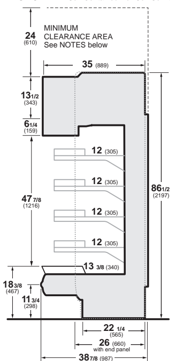
RGDC 24-72 Self-Contained Deli Self-Service
