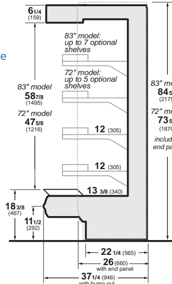
RGDC24 deep, 72" or 83" high Remote Refrigerated Gondola Display
