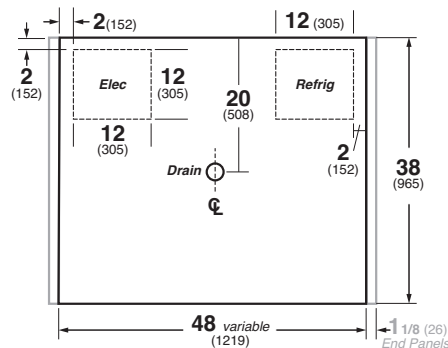
SGB Plan View
