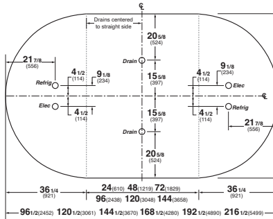
TY4-6X(case length) I - Island Merchandiser
