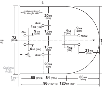
TY4-6X(case length) E - Flat End Merchandiser
