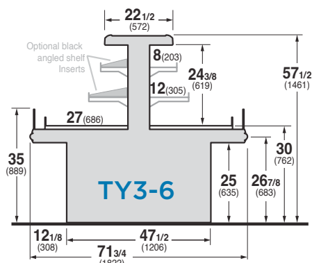
□ 6'x8' island (TY3-6X8I-SA)
