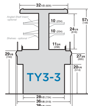
□ 3'x4.5' end (TY3-3X45E-SA)
