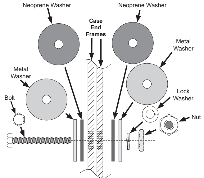
Detail for Connecting Merchandiser End Frames
