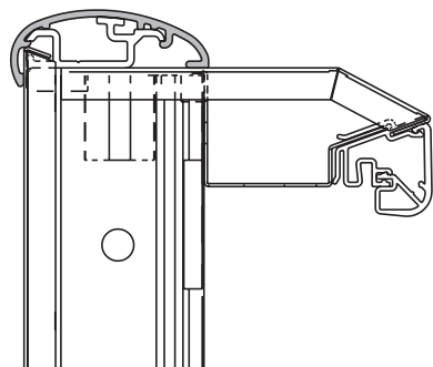
Hand Rail Snapped onto Retainer
