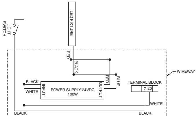
2 DOOR END COMPARTMENT LED LIGHT WIRING DIAGRAM
