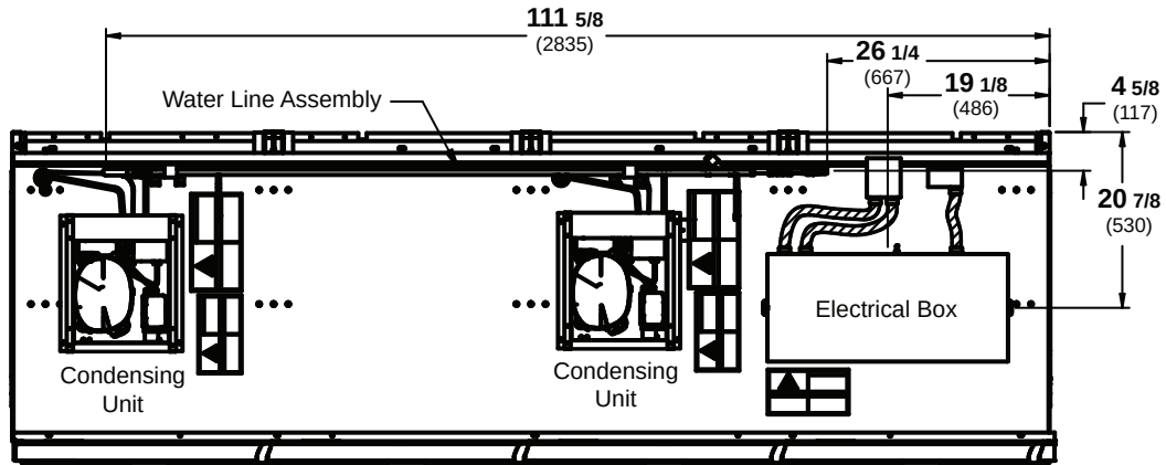
RL4SP Top View
