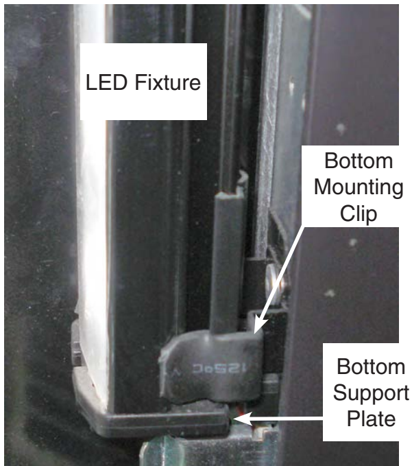
Figure 4. Bottom Support Plate and Clip (End Fixture Shown, Center Fixture Similar)
