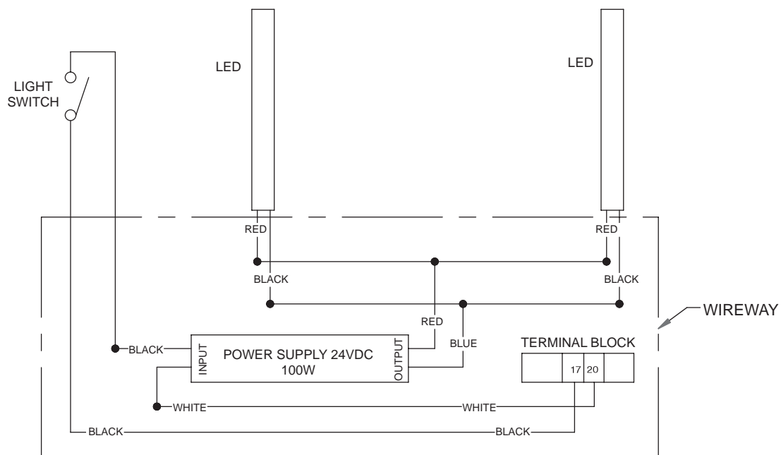
1 DOOR LED LIGHT WIRING DIAGRAM
