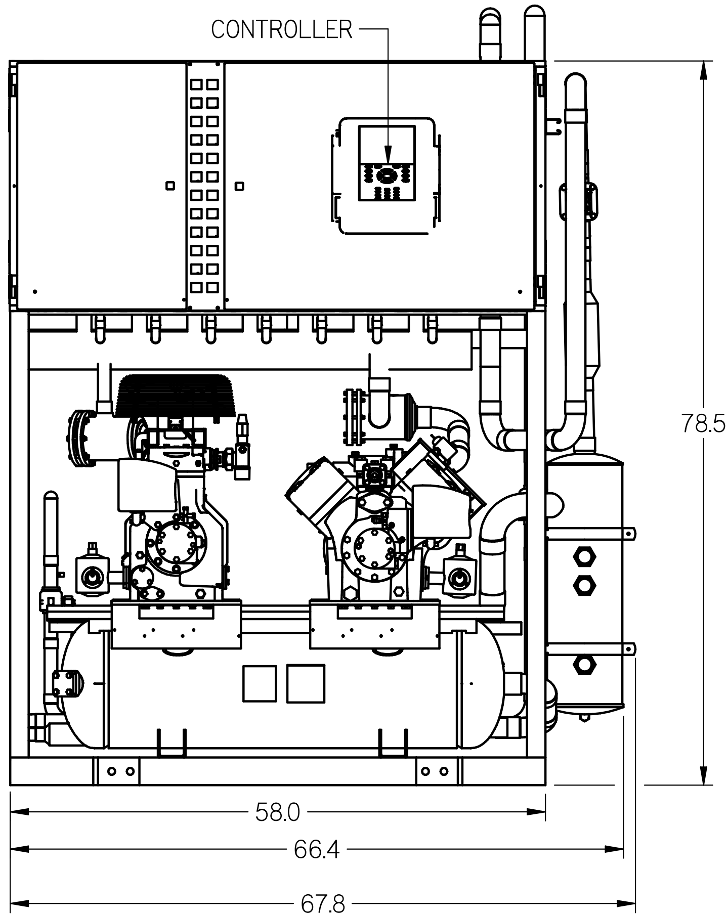
RACK DIMENSIONS: 66"L X 39"W X 78.5"H
