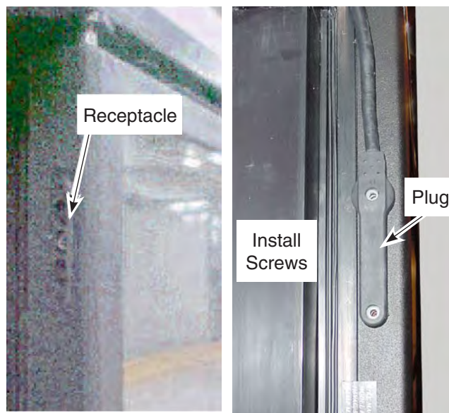
Connect Heater
