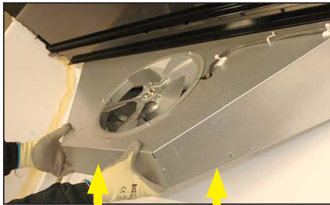
Lift up Fan Plenum. Use chain to hook up fan plenum to facilitate cleaning (for inside wedges).
