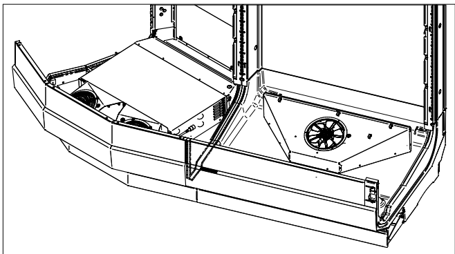
Apply Neutral Curing Silicone Sealant Outside Wedge Case
