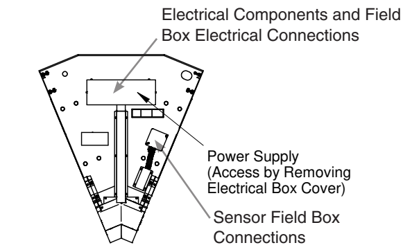
45° Inside Wedge Case
