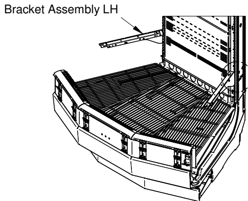
Shelf Bracket Assembly
