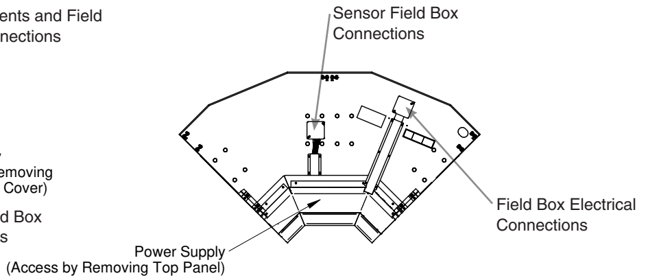
90° Inside Wedge Case
