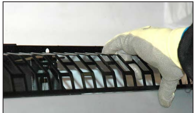
Lift up Fan Plenum. Use chain to hook up fan plenum to facilitate cleaning (for inside wedges).
