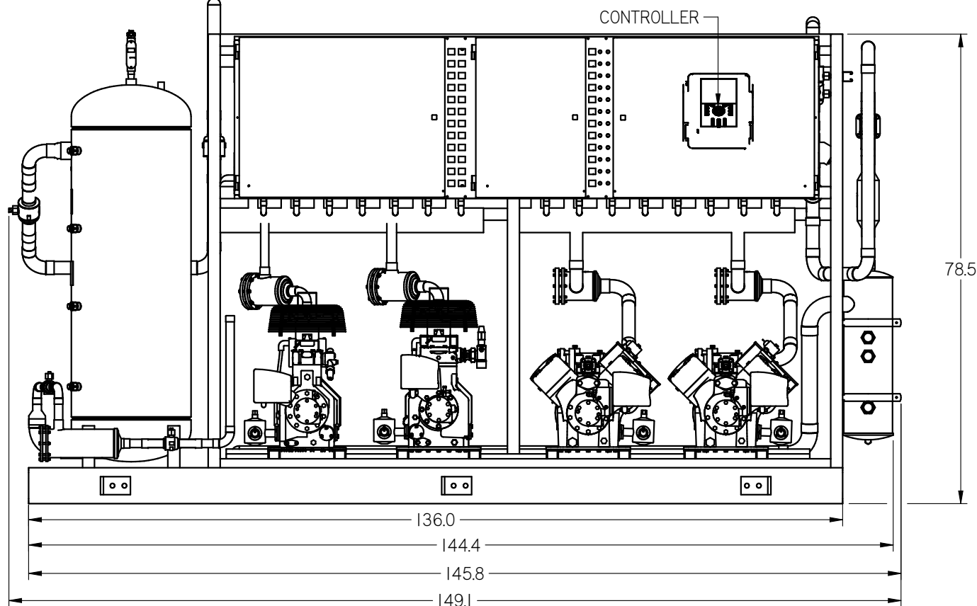
RACK DIMENSIONS: 144"L X 39"W X 78.5"H
