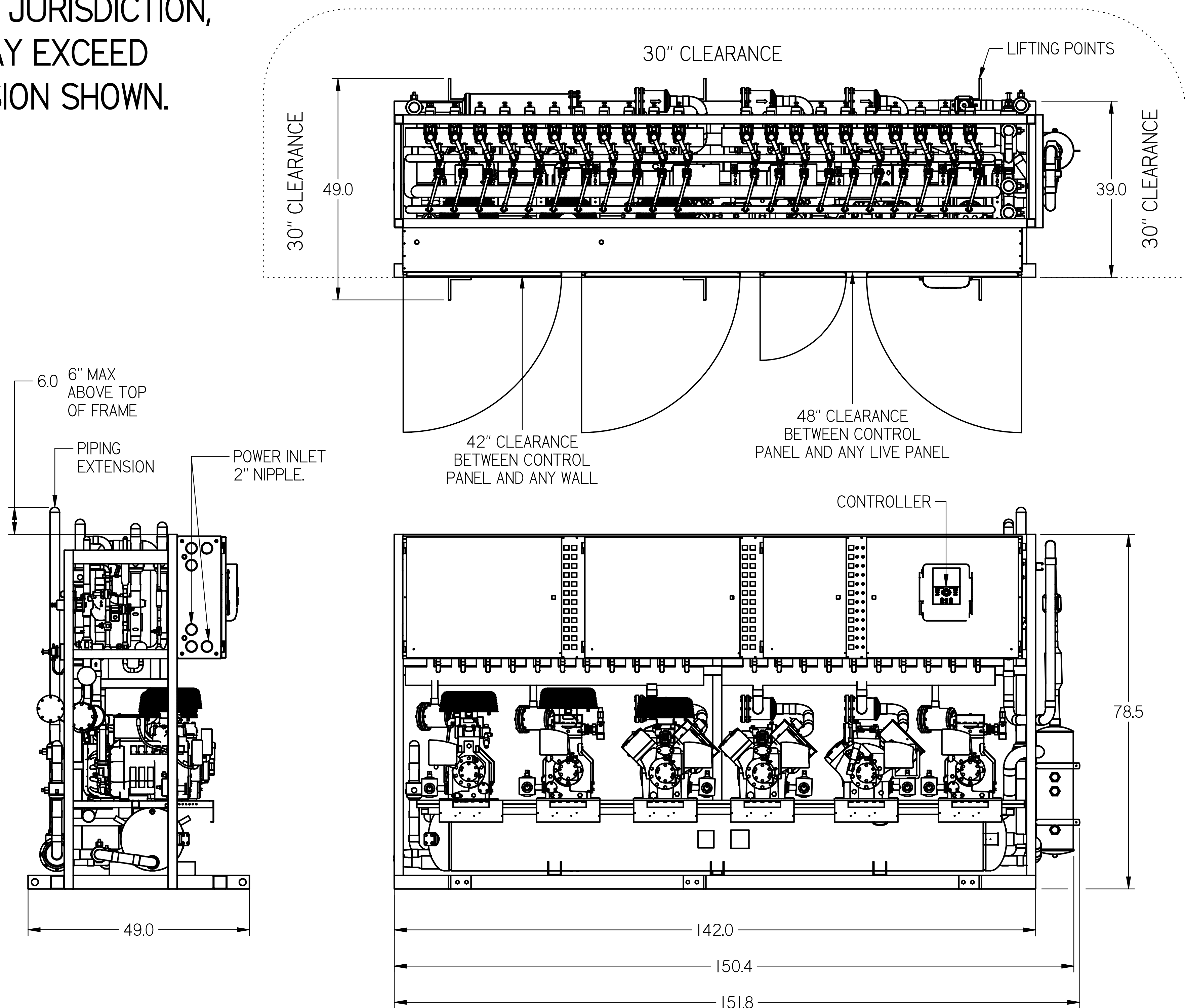
RACK DIMENSIONS: 150"L X 39"W X 78.5"H
