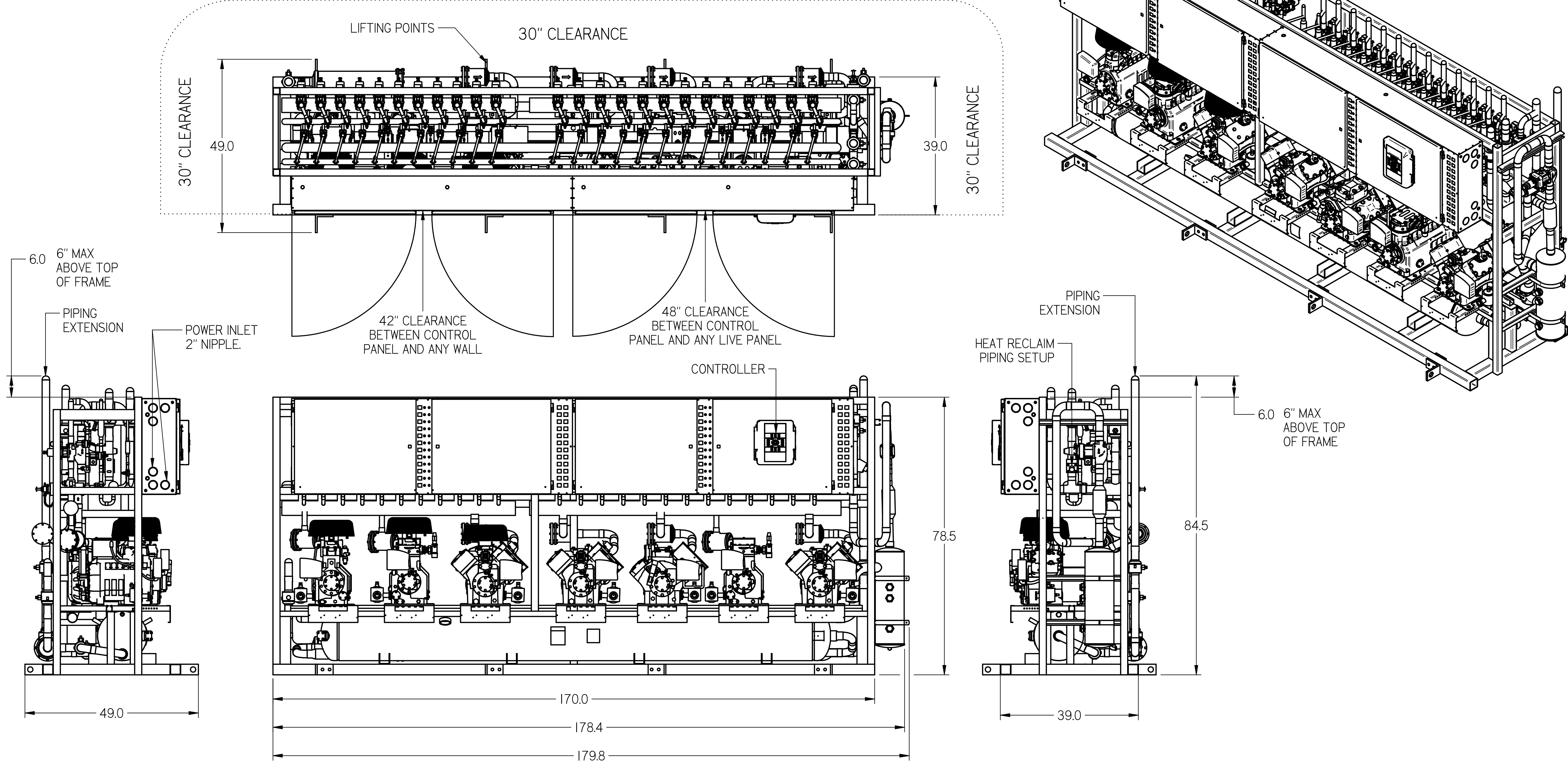
RACK DIMENSIONS: 178"L X 39"W X 78.5"H
