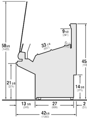
DSFM with Straight glass
