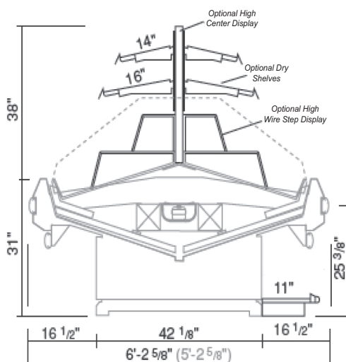
DSRPI-03 Shelf & Rack Option Scale = 3/8"
