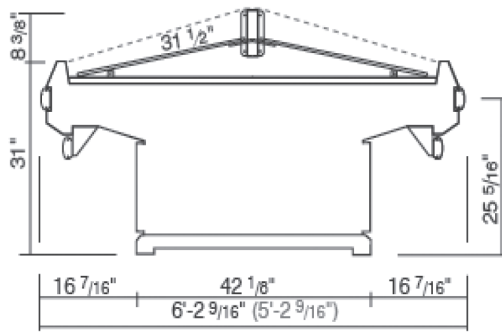
DSI-03, DSI-03Y (Impact) Standard Section Scale = 3/8"
