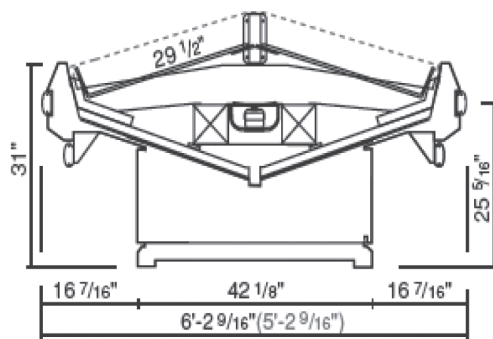
DSRPI-03, DSRPI-03Y (Impact) Standard Section Scale = 3/8"
