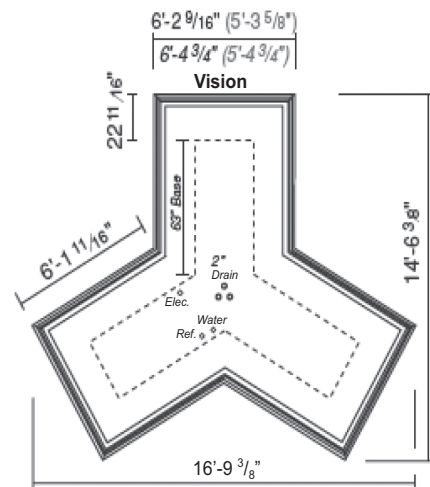
DSRPI-03Y (Impact) Plan View Scale = 1/8"
