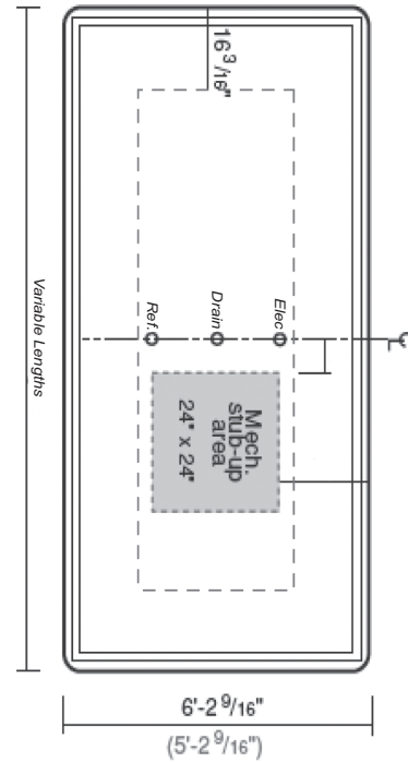
DSRPI-03 (Impact) Plan View Scale = 1/4"
