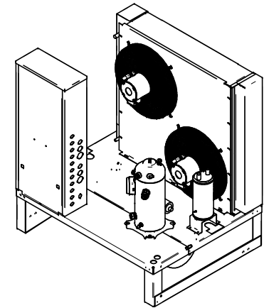
ISO VIEW
