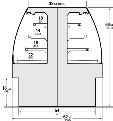
IM-04-Tx-S Back-to-Back Multi-Deck Self-Service Self-Contained
