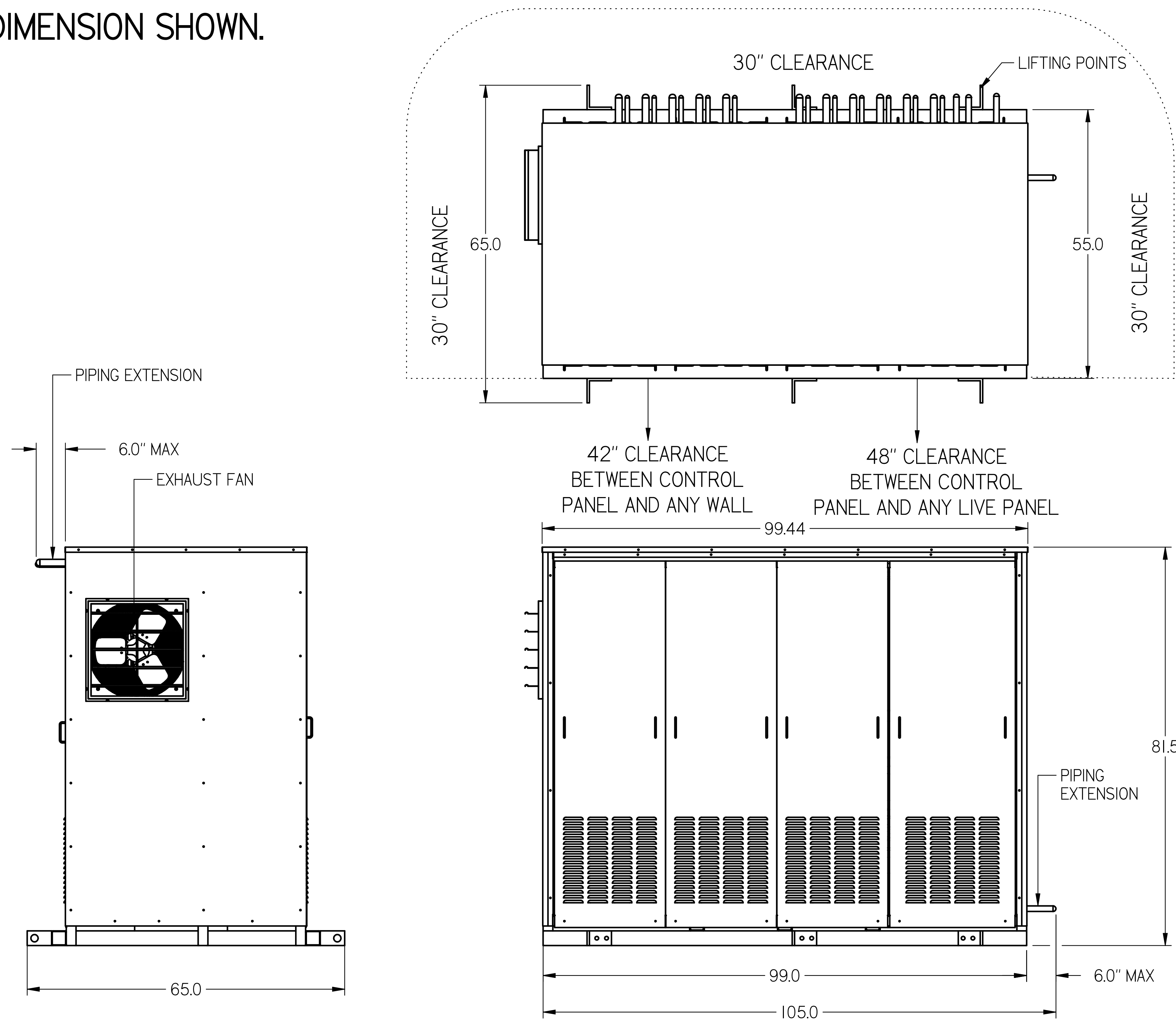
RACK DIMENSIONS: 99"L X 55"W X 81.5"H
