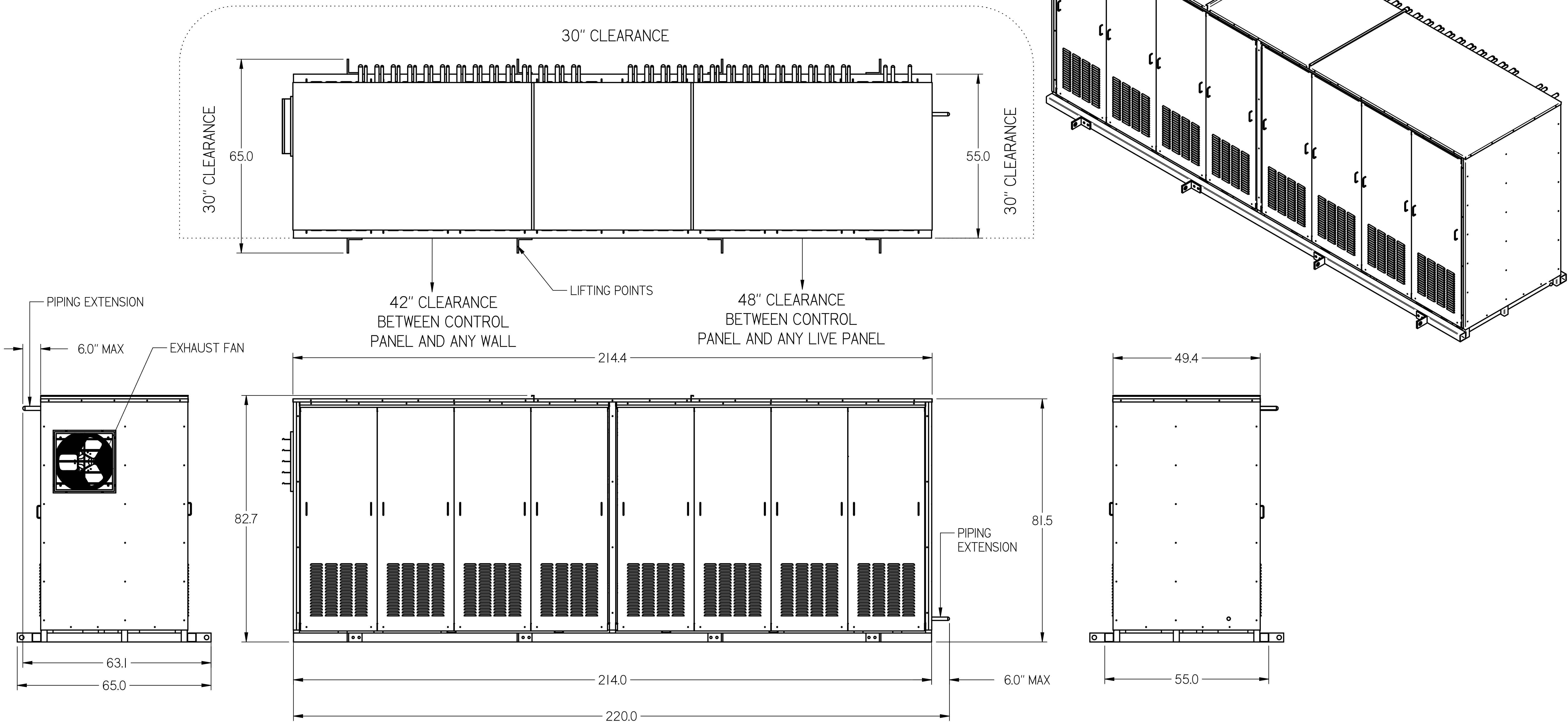
RACK DIMENSIONS: 214"L X 55"W X 81.5"H
