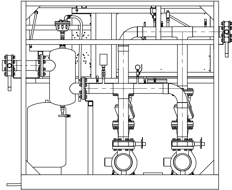
BACK VIEW
