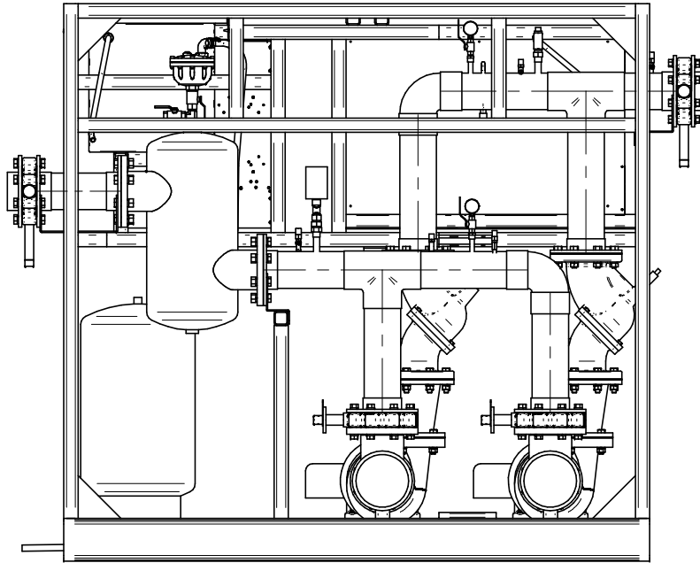
BACK VIEW
