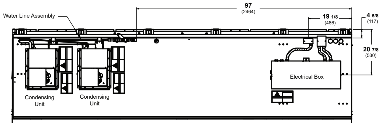
RLN5SP Top View
