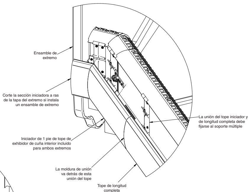
Exhibidor de cuña interior
