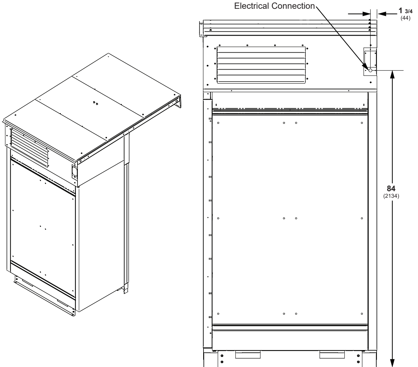
Back of Module (Dimensions to Rear Junction Box)
