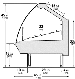
Curved Glass - Single-Deck Fish
