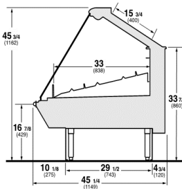
Straight Glass - Single-Deck Fish
