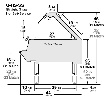
SELF-SERVICE CASE W/HEATED DECK
