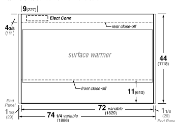
QH-SS Q-Series Hot Merchandisers
