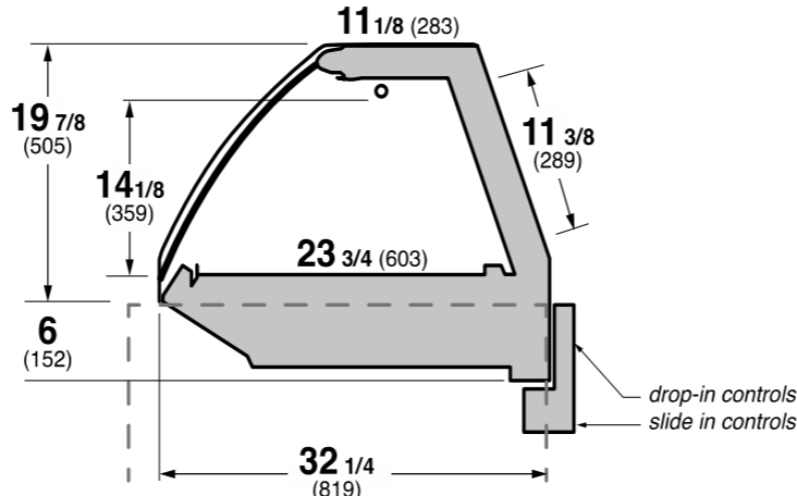
CR3TO Refrigerated Drop-In Counter-Curved Glass
