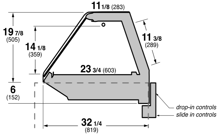
R3TO Refrigerated Drop-In Counter
