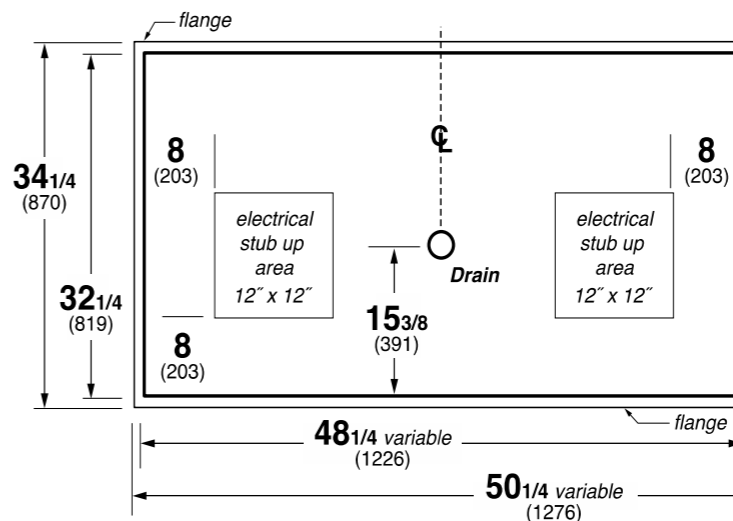
R3TO / CR3TO Plan View
